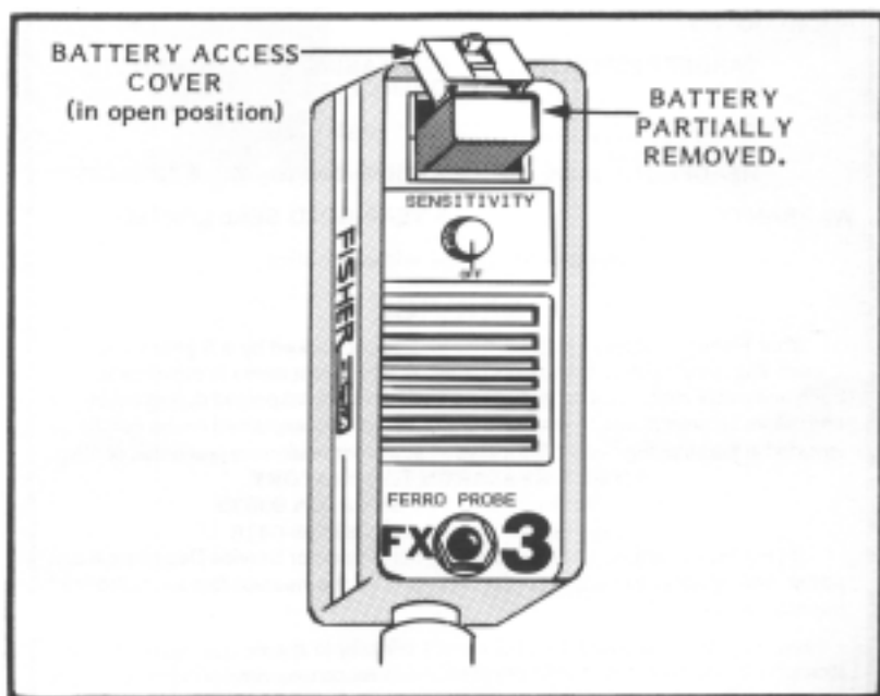
Figure 8. Battery Replacement
