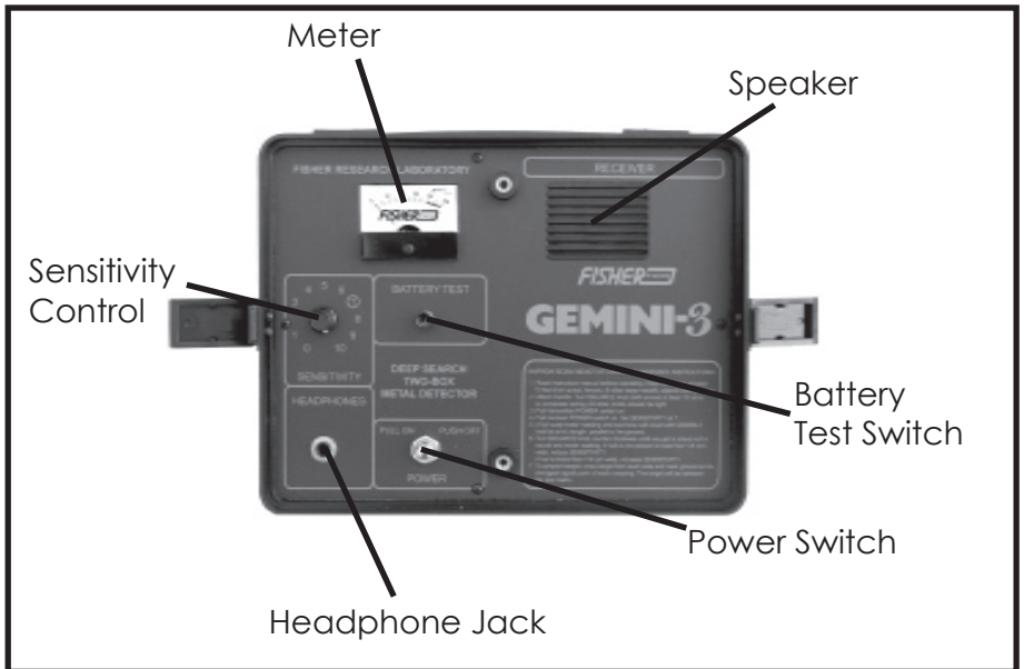
Figure 3. Receiver
