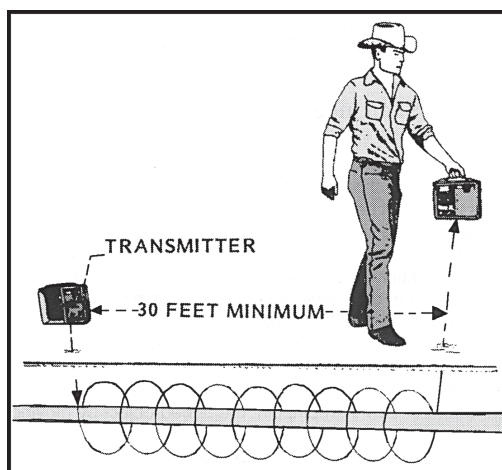
Figure 8. Inductive Trace
