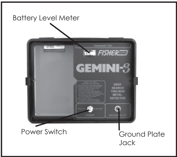
Figure 2. Transmitter
