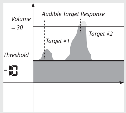
If the Threshold is set to a positive value, high enough for you to hear the faint hum, the detector will produce target signals and a Threshold sound. It is recommended that you set a Threshold that is still very low; a high Threshold can mask small target signals.
